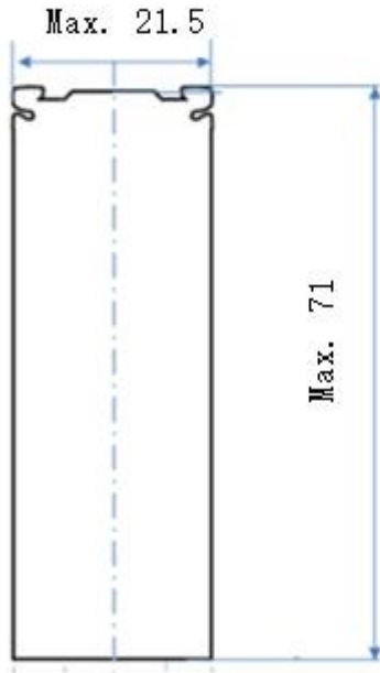
Fig. 2 outline dimensions of ICR21700-48G
