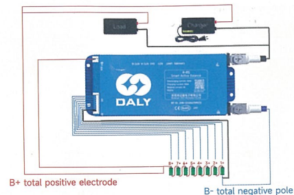
4-8S BMS 8S wiring diagram
